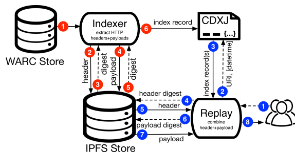
Figure 2: The ipwb indexer and replay workflow.
